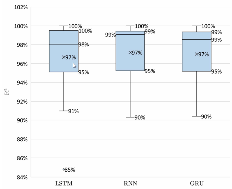
(b) ANN-based Models
