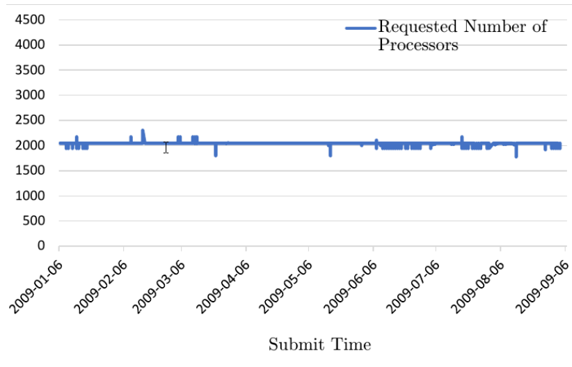
Figure 4.9: Extracted pattern from ANL-Interpad trace attribute
