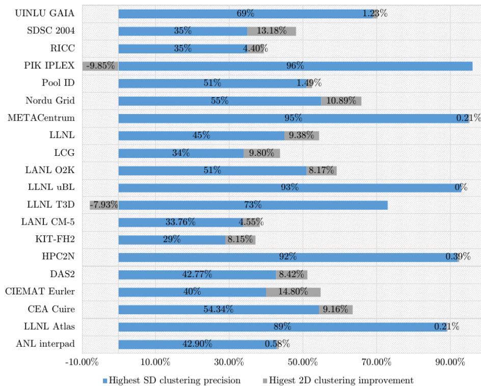
Figure 2.7: Highest improvement from single-attribute (SD) to dual-attribute (2D) clustering across all applicable traces
