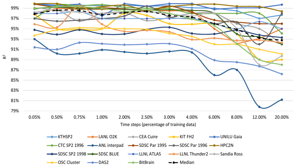
Figure 4.14: Confidence range of the MICRAST approach over time
