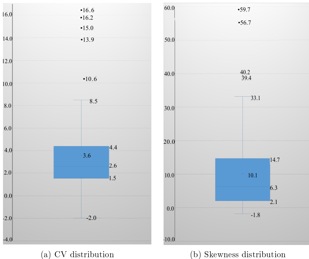
Figure 4.3: Ranges of statistical distributions for supervised traces
