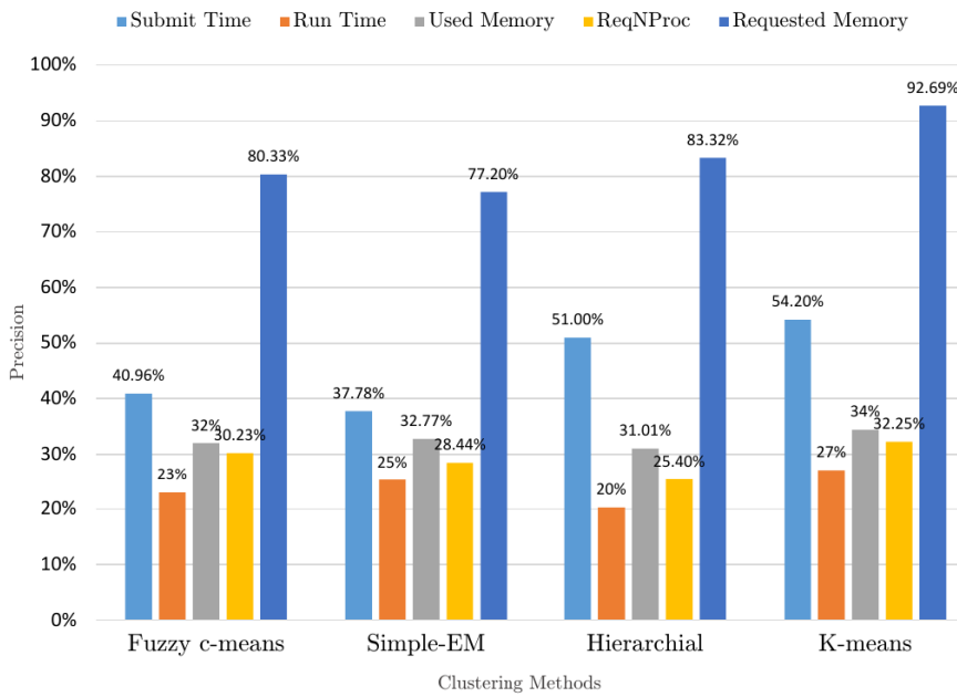
Figure 2.5: Sample showing the impact of method selection on clustering quality in the HPC2N-2002 trace
