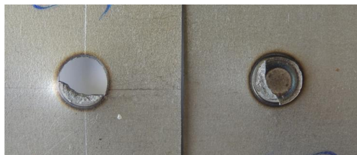
Figure 7.6. Partial plug failure mode in sample C3 of MS1400.
