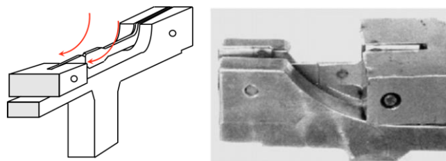
Figure 3.11. The fixation of the specimen to the special specimen holder [163]
