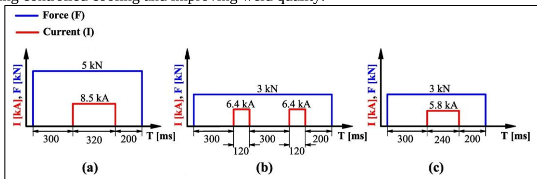
Figure 8.1. Schematic of RSW Schedules. (a) long-tome (Hard work), (b) 2-pulse (Post-heat work), and (c) short-time RSW (Soft work)
