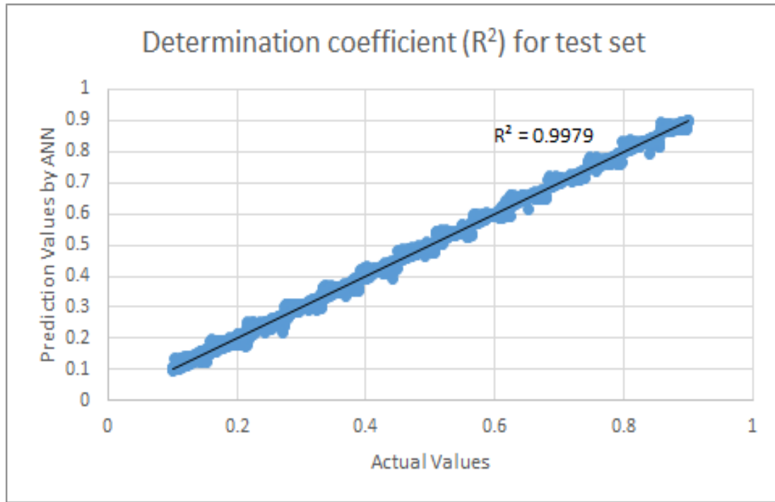
Figure 7.7. Neural network performance determination coefficient – test set
