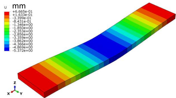
Figure 9.16. Deflection of the structure in case of 6 layers in the face sheets
