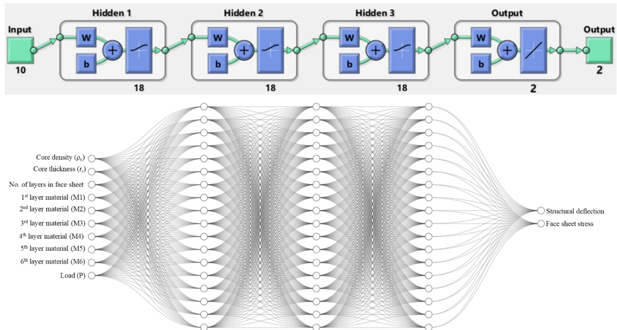
Figure 9.3. Neural network structure for the investigated sandwich structure
