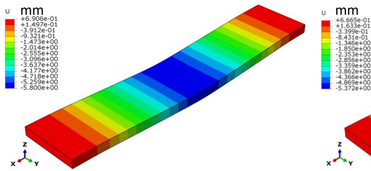
Figure 9.15. Deflection of the structure in case of 5 layers in the face sheets
