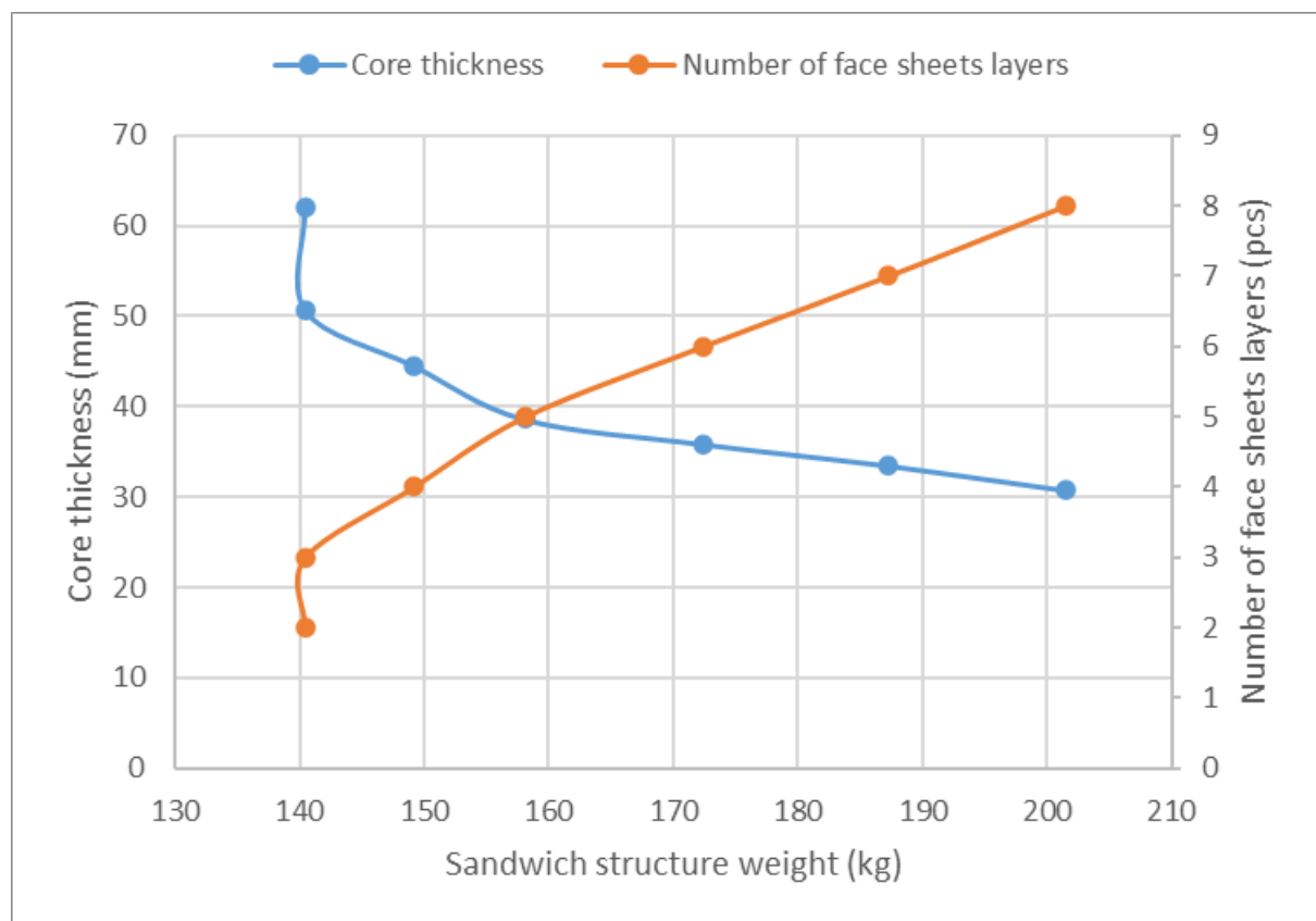
Figure 4.2. Weight of the sandwich structure versus core thickness and face sheets' layer number in case of WGFPR face sheets and Al honeycomb core
