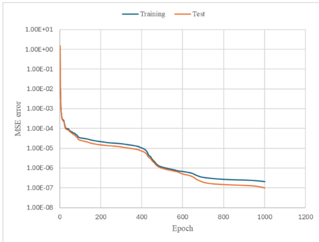
Figure 9.10. Mean Square Error (MSE) for the ANN in case of investigated structures
