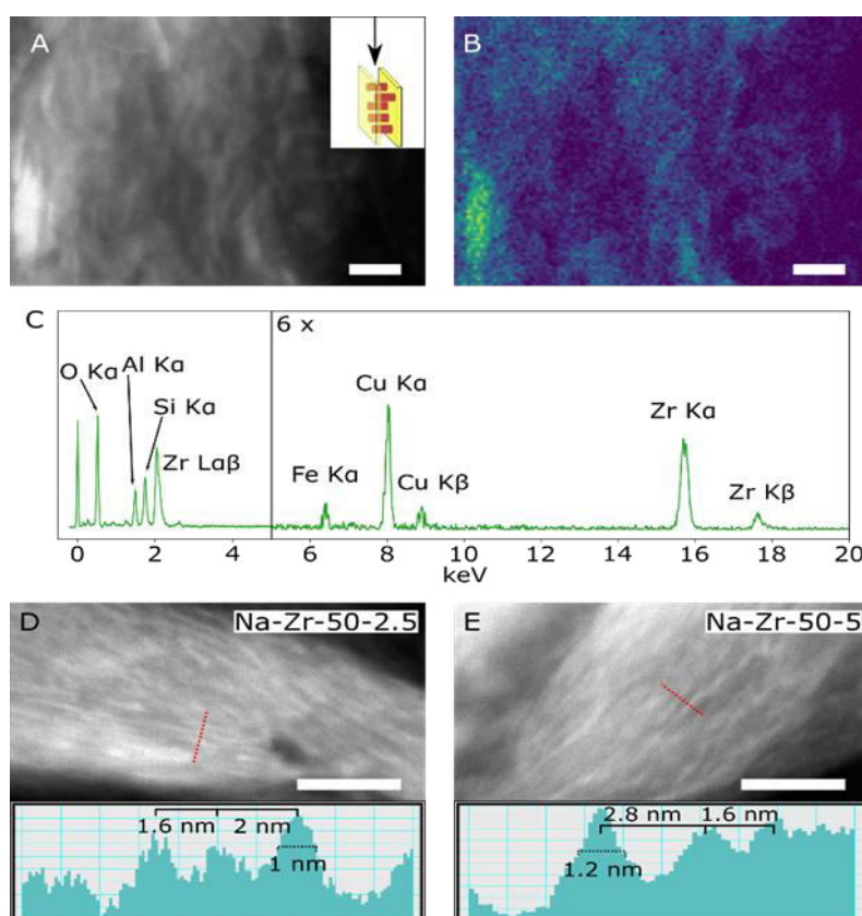
Figure 15: The similarities between the STEM-HAADF ( A ) and STEM-EDX map of Zr-rich areas ( B ) in Zr-50-10 show that the bright fringes in the HAADF images can be correlated to areas rich in Zr. The inset in ( A ) illustrates the viewing direction, where the intercalated \text{ZrO}_2 layers are parallel to the electron beam. ( C ) The NMF-component used to construct B is dominated by Zr, but additionally contains the Al and Si from the surrounding clay. Additionally, higher resolution HAADF images of Na-Zr-50-2.5 ( D ) and Na-Zr-50-5 ( E ) with inset line profiles exemplify the relative size and spacing of the fringes. The scale bars in each image represent 20 nm.
