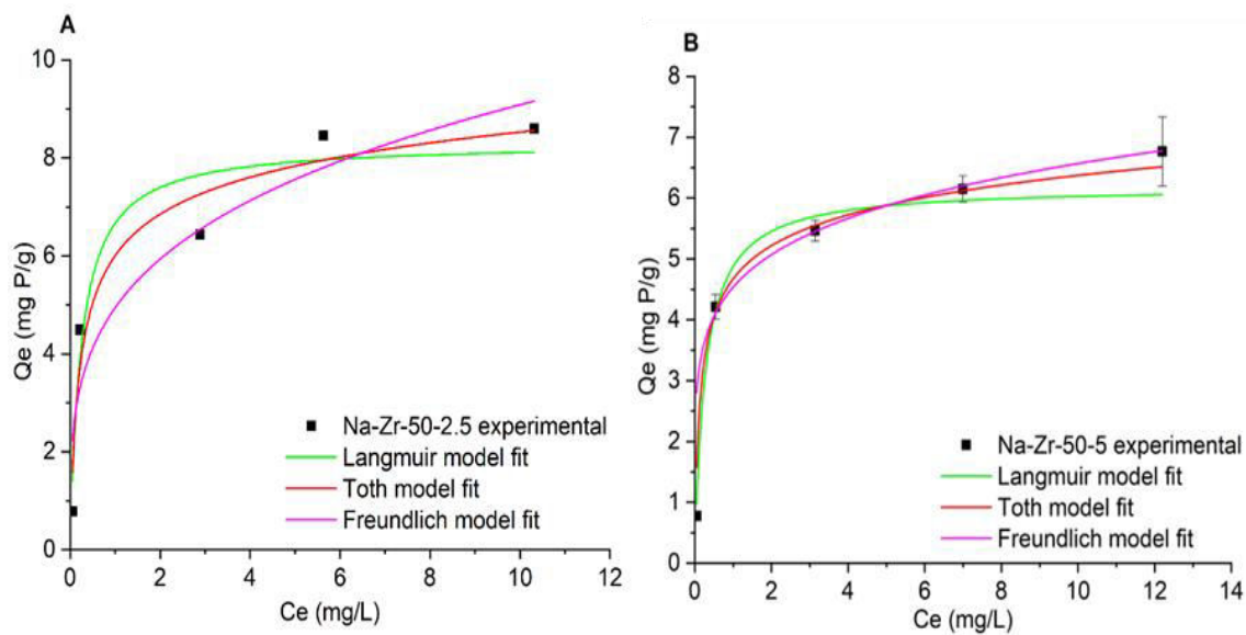
Figure 21: Adsorption isotherms of phosphates on Zr-pillared clays at pH 7.
