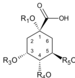
Kinasav
